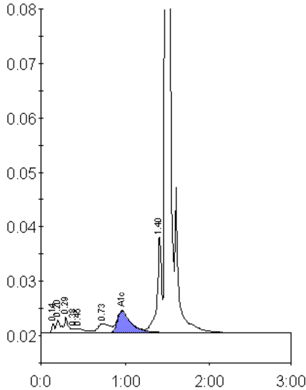
Peak table - ID: 10583680
